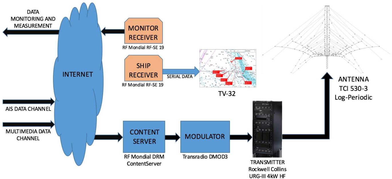
Figure H-2. Field test equipment set-up.
