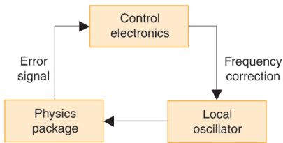
▲ FIGURE 1 The three subsystems of a passive frequency reference and the interaction between them.
