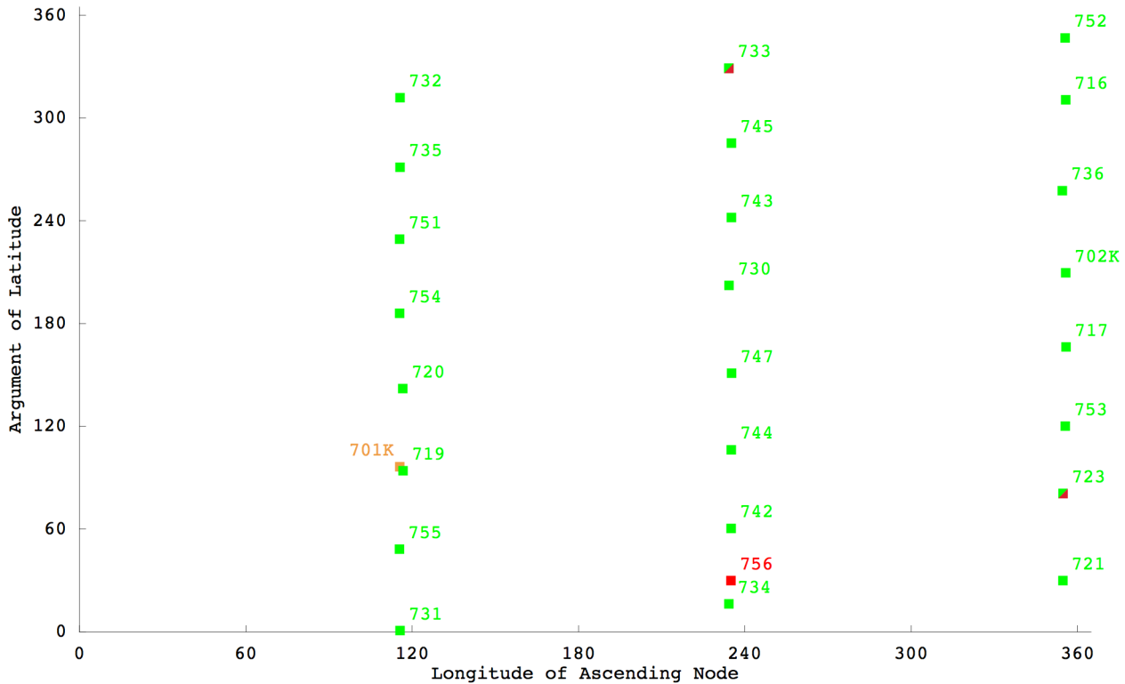
GLONASS Satellite Constellation (GPS Week 2010(986); GPS Seconds 259200)
