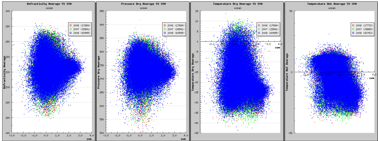
Figure 2: Correlation between the reflection flag (Ocean events) and atmospheric parameters extracted from the post-processed RO profiles (averaged at the bottom 5-km). Left-to-right: refractivity; dry pressure; dry temperature; wet temperature.
