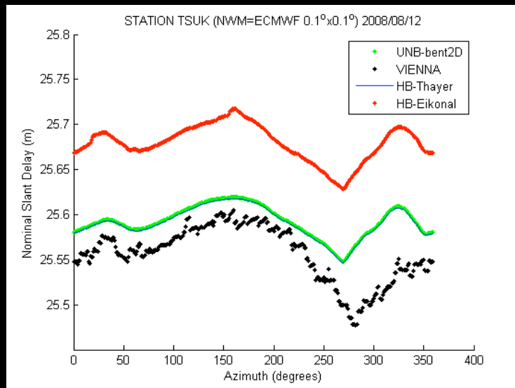
Slant delay at 5° elevation angle for various ray-tracing algorithms
