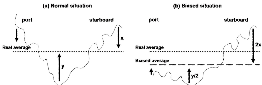
Figure 2.28 (a) Normal situation when amplitudes are equally distributed for both sides. (b) Biased situation when lower port side averages pulls averages downwards.
