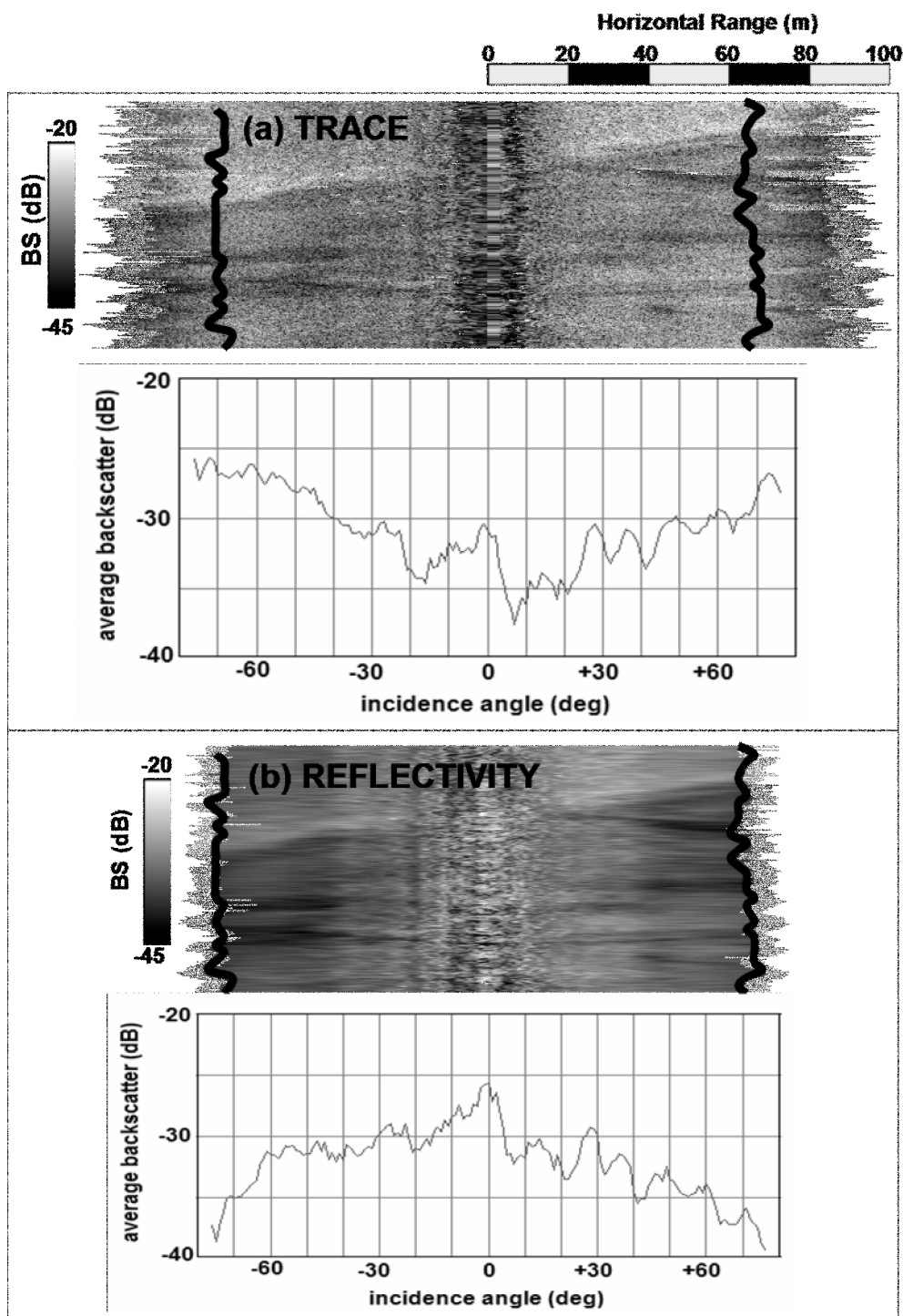
Figure 2.13 (Top Image) Full sidescan trace data logged in the sonar image amplitude telegram and its average backscatter taken with getBeamPattern software. (Bottom Image) Beam average reflectivity data logged in depth telegram. Notice better resolution and extended area coverage of full trace data. Average backscatter plots have inverted pattern because reflectivity data is not compensated for the angular response effect.
