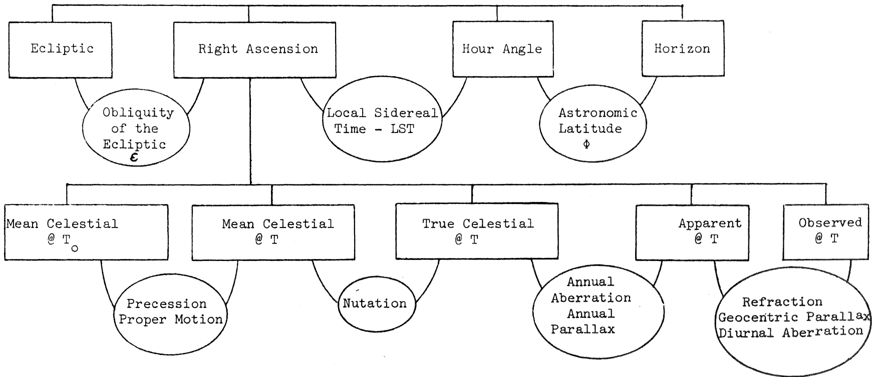
Figure 3-11. Celestial Coordinate Systems.
