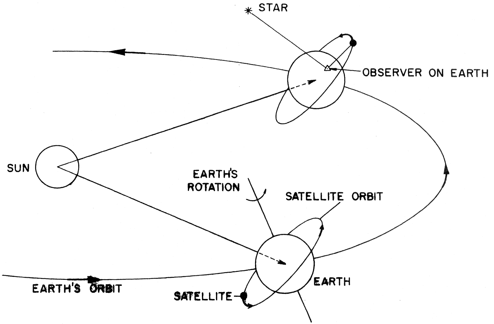
TERRESTRIAL , CELESTIAL AND ORBITAL COORDINATE SYSTEMS.
