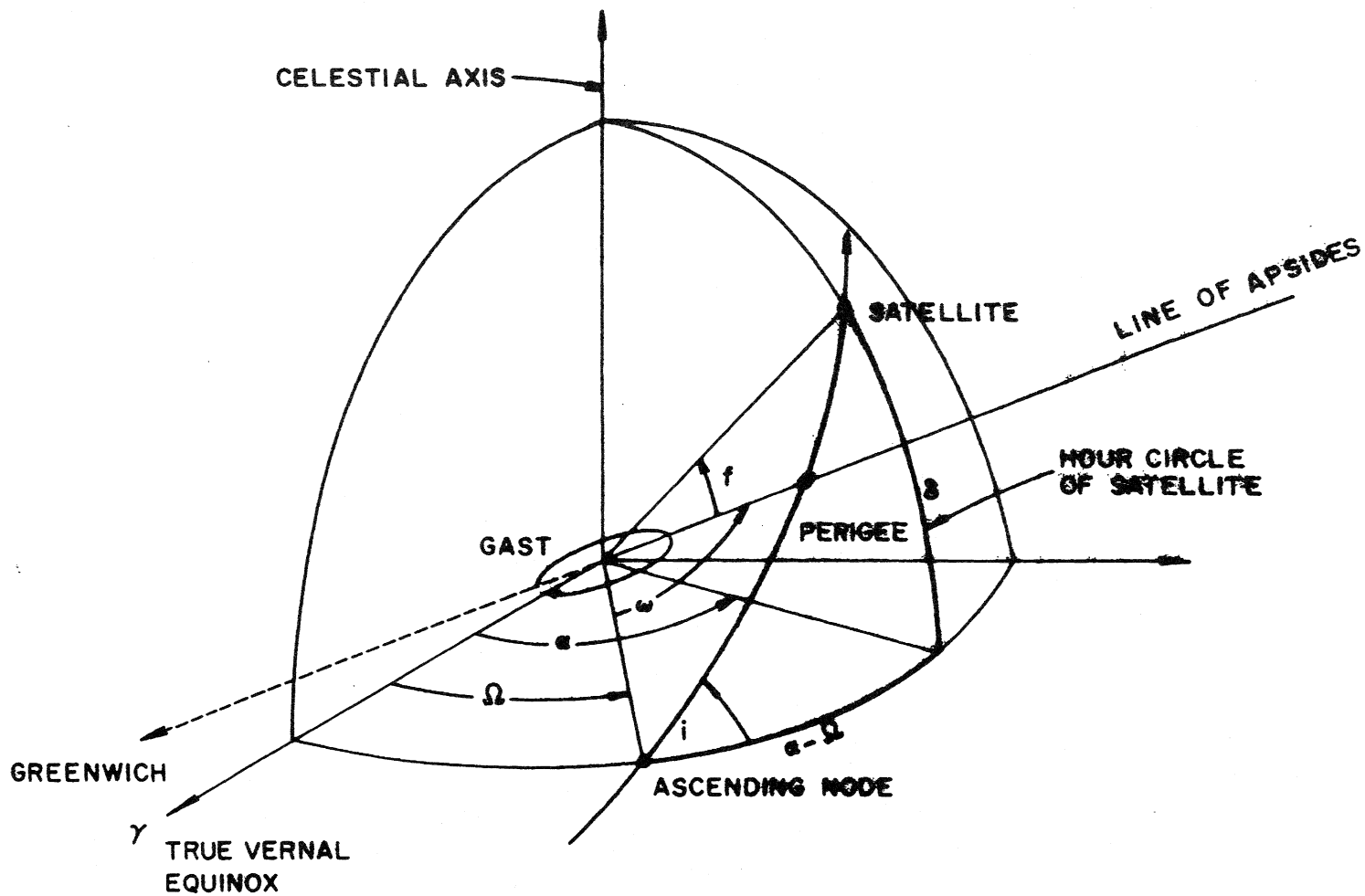
FIGURE 4-2 KEPLERIAN ORBITAL ELEMENTS
