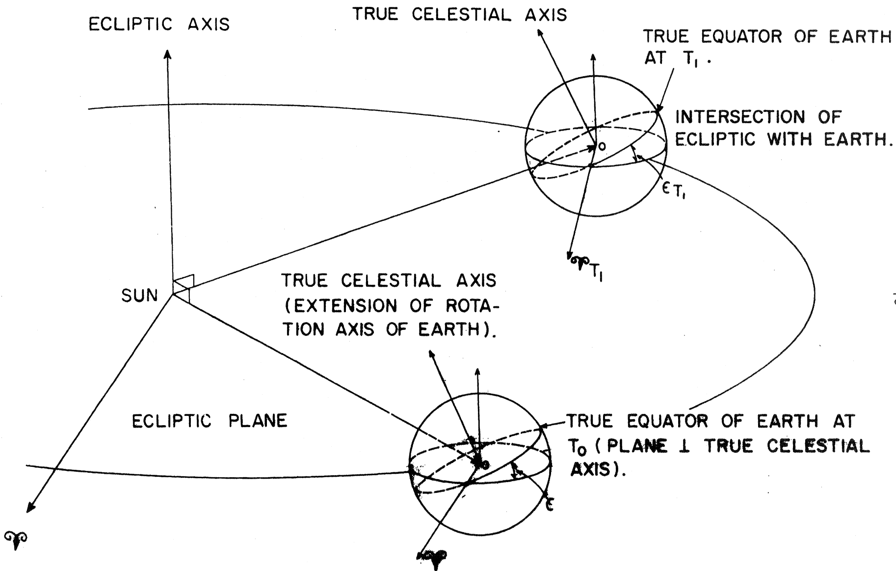
Figure 3-8. THE EFFECT OF PRECESSION AND NUTATION
